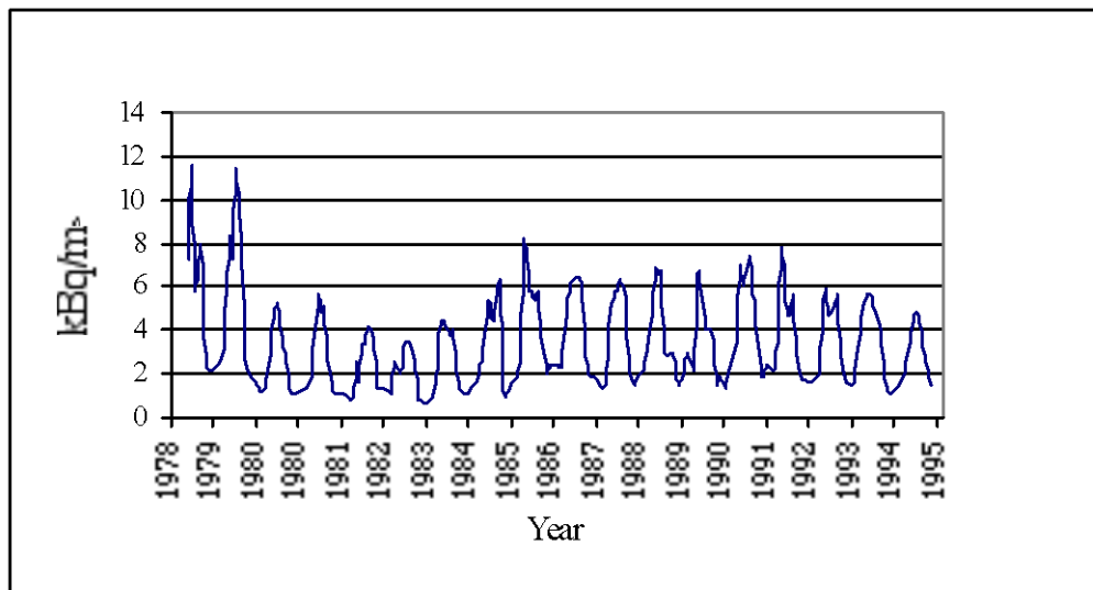
Fig. 2 - Radon concentration in Hajnóczy Cave (Hungary) (Hakl et al., 1995)
