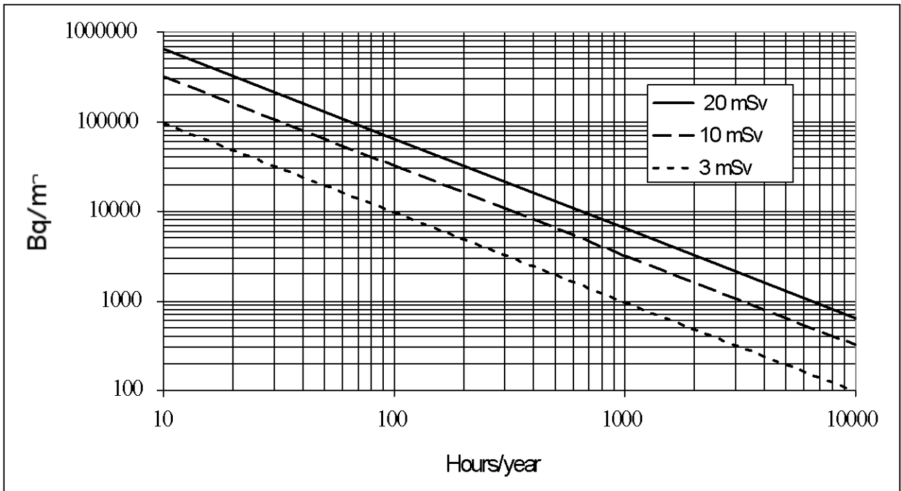
Fig. 6 - Hours per year which can be spent with annual dose limits of 20, 10 and 3 mSv respectively and an equilibrium factor of 0.4.
